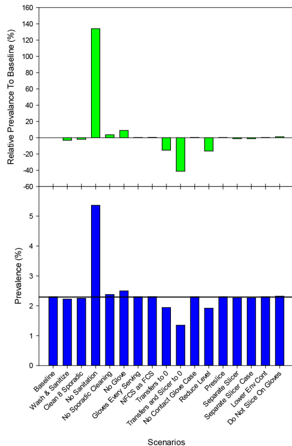
Figure 17: Effect of various sanitation scenarios on the prevalence and relative prevalence of L. monocytogenes -contaminated RTE products in a retail deli with multiple niches
